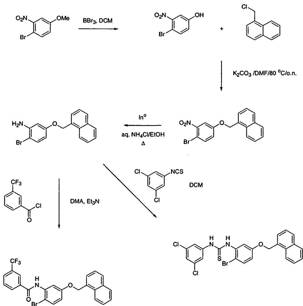
Scheme VII
